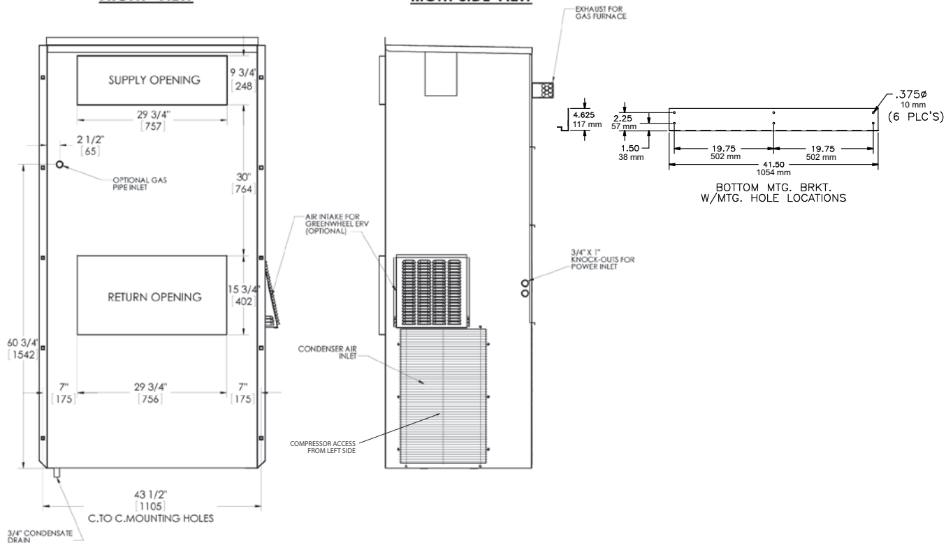
REAR VIEW
