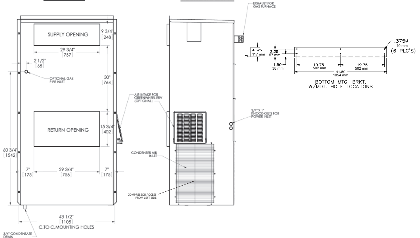
REAR VIEW
